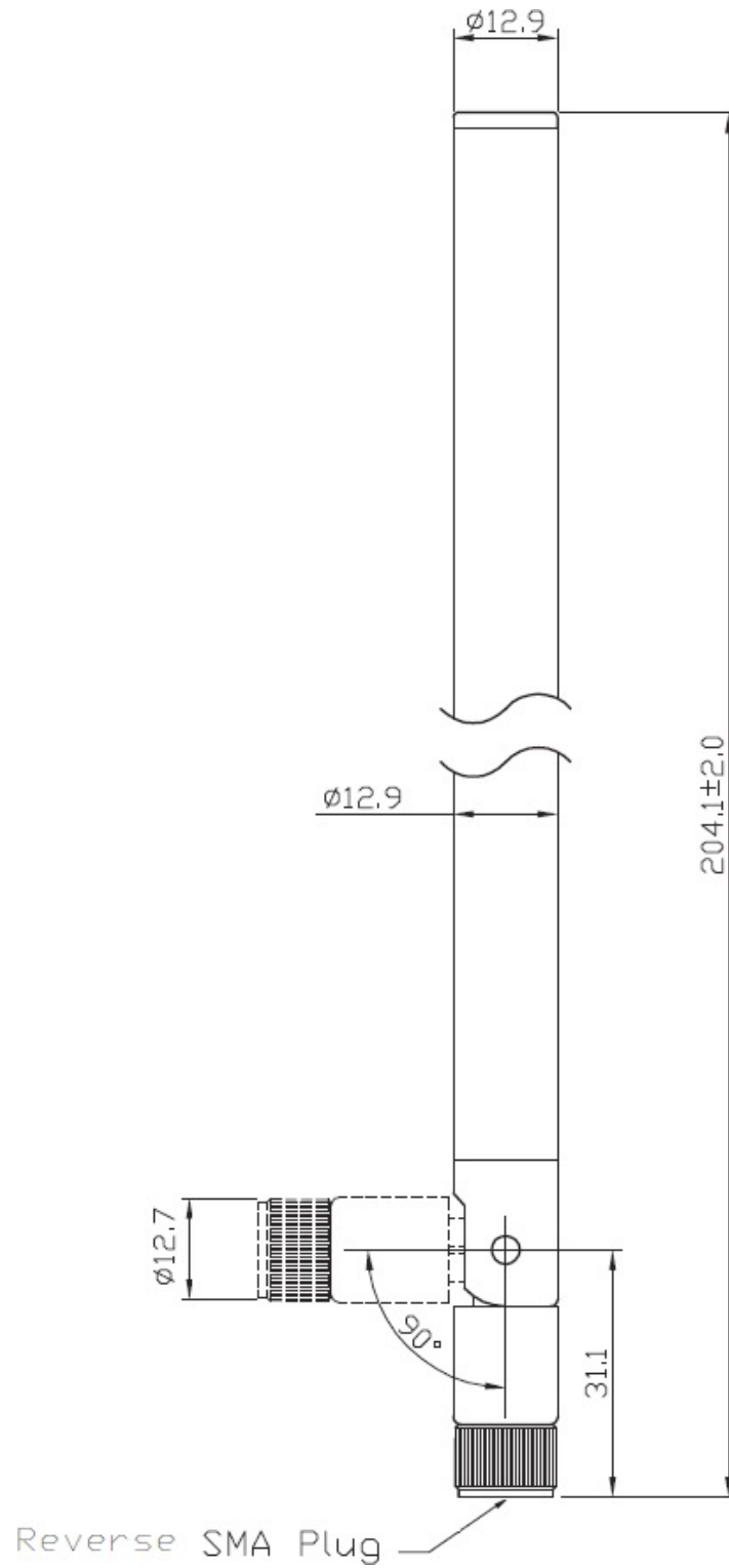
Figure 1 Physical Dimensions
