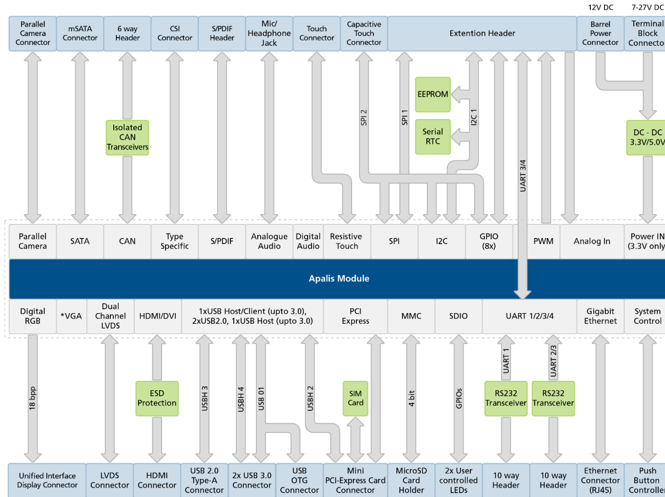
Fig.1 Ixora Carrier Board Hardware Architecture
