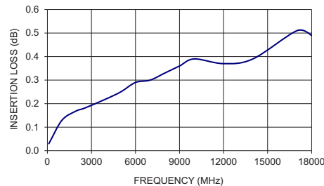
047-3SMPR+ INSERTION LOSS
