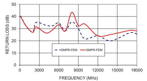
047-3SMPR+ RETURN LOSS
