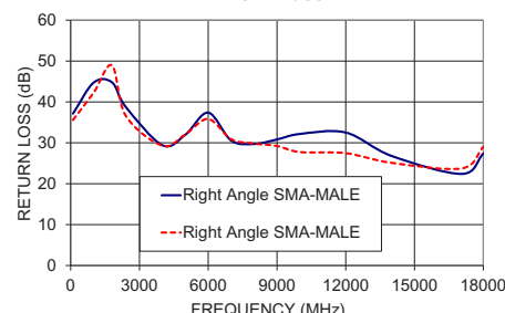
086-14SMR+ RETURN LOSS
