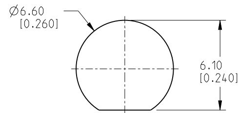
RECOMMENDED MOUNTING HOLE DIMENSIONS
