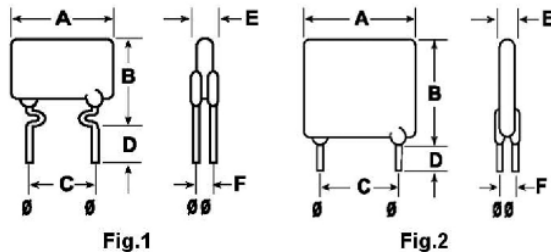
Lead Size : 24AWG Φ0.51 mm Diameter
