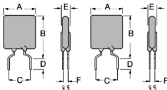
Fig.3 Lead Size : .20AWG Φ 0.81 mm Diameter
