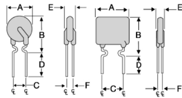
Fig.1 Lead Size : .24AWG Φ0.51 mm Diameter
