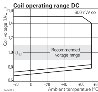
S0530-B
