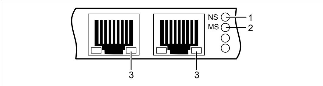
Fig. 8 LEDs EtherNet/IP
