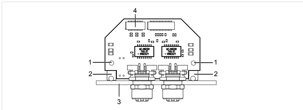
Fig. 2 Mounting guides
