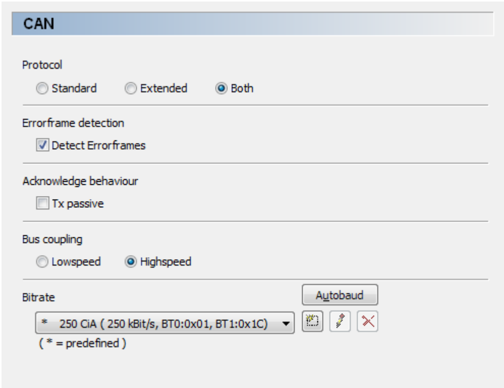
Figure 5.13: CAN Settings
