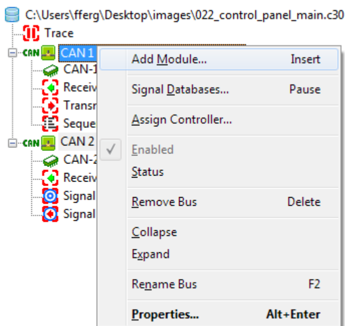
Figure 5.4: Configuration tree of the control panel
