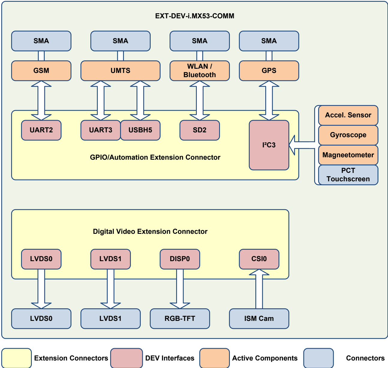
Figure 2-1: Interconnection Diagram
