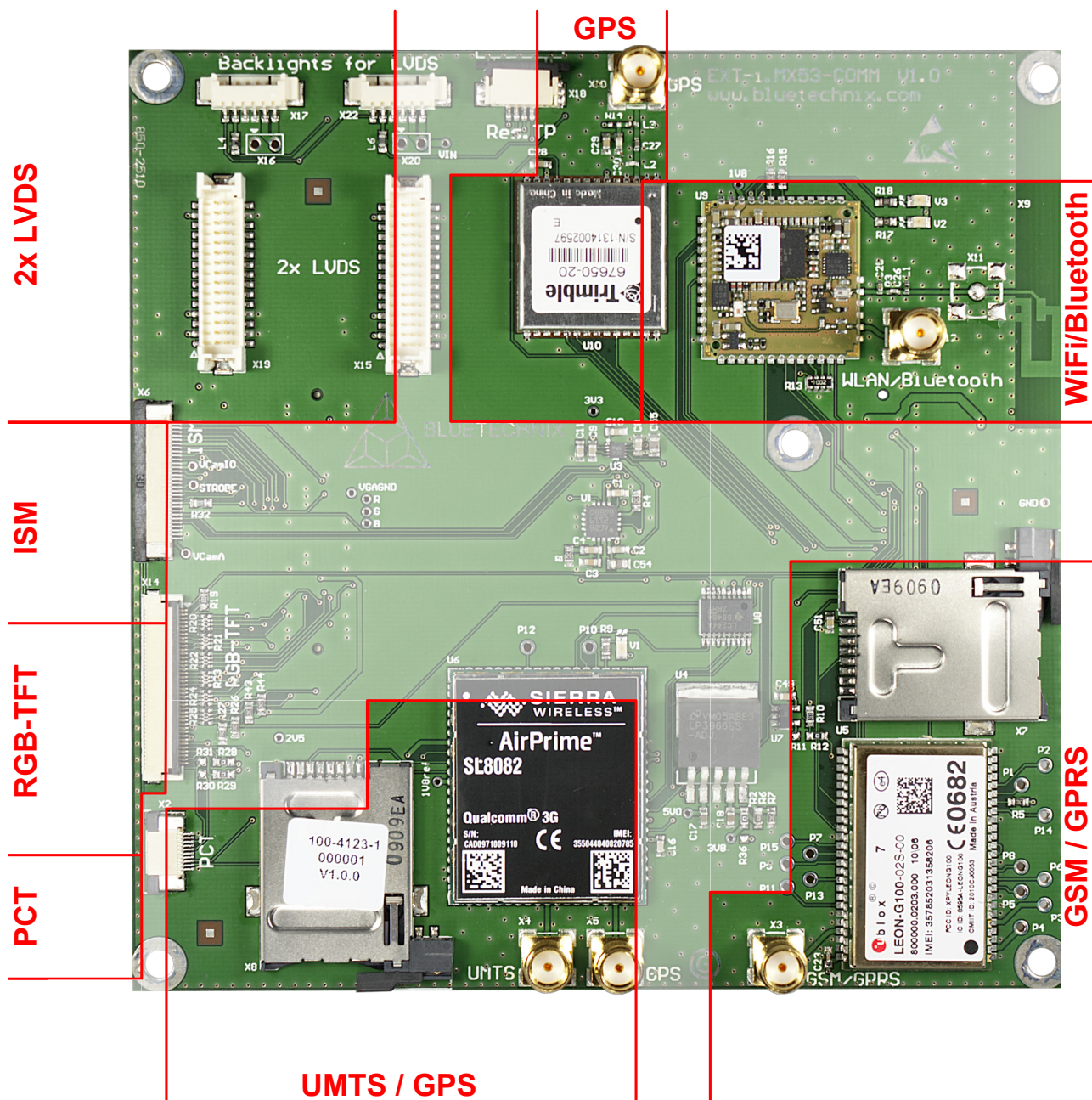
Figure 4-1: RF-Module and Connector Location
