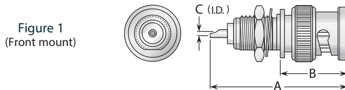
Bulkhead Plug Receptacle
