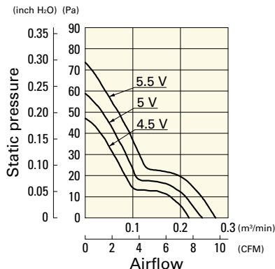
109P0405F3013 With pulse sensor
