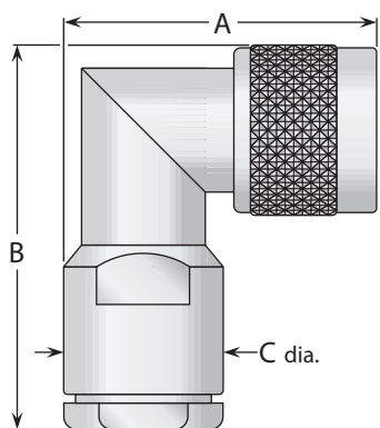
Figure 1 (Mitered body)
