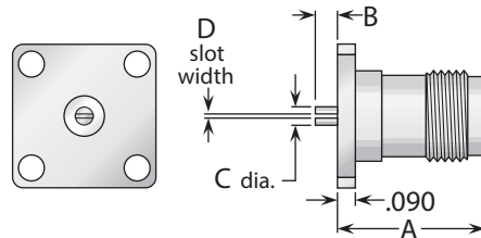
Figure 2 (Slotted contact)
