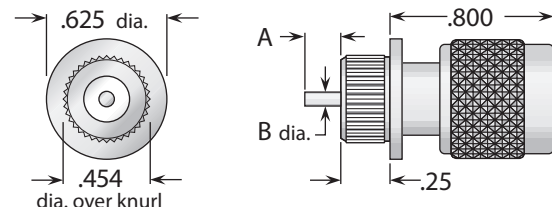
Figure 4 (Plug type, post contact)
