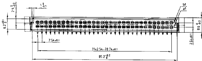
PCB-hole pattern
