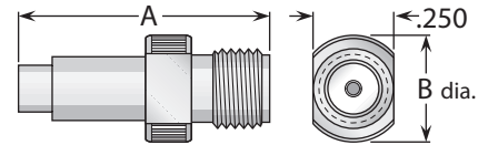
Figure 2 (Straight jack)
