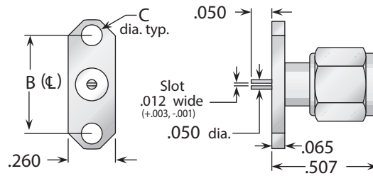
Figure 3 (2-hole flange)
