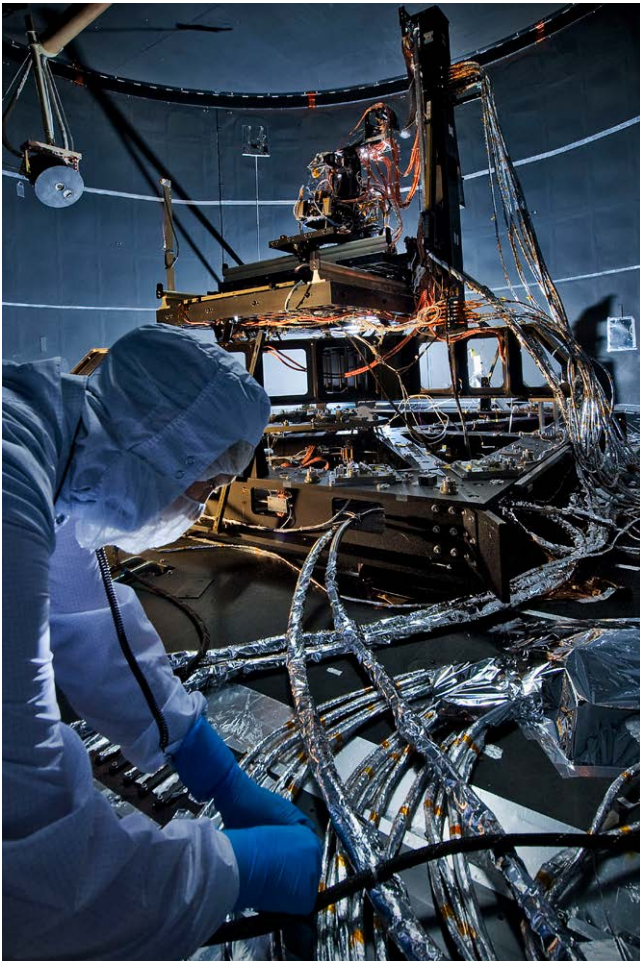
Thermal-vacuum chamber
