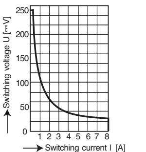
Safe disconnection, no remaining arc, max. 1 operation/sec. Maximum switching power curve
