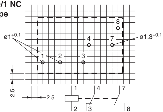
1 NO/1 NC, S-Type
