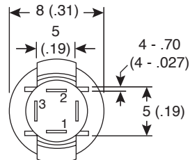
Mounting Hole Dimension
