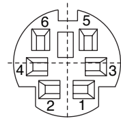
6-Pin 161-2306
