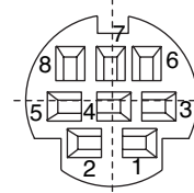
8-Pin 161-2308
