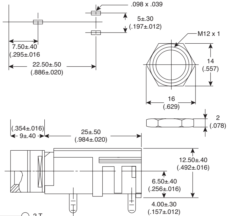
DIMENSIONS: mm (in.)
