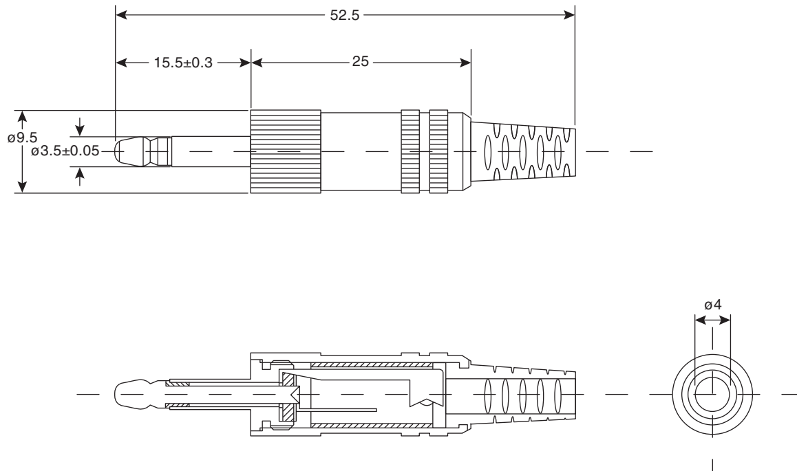
Dimensions: mm
