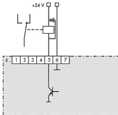
RELAY CONTROL
