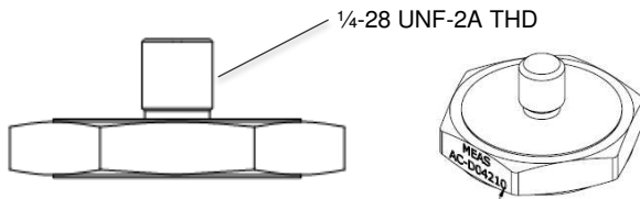
Adhesive Mounting Stud P/N AC-D04210
