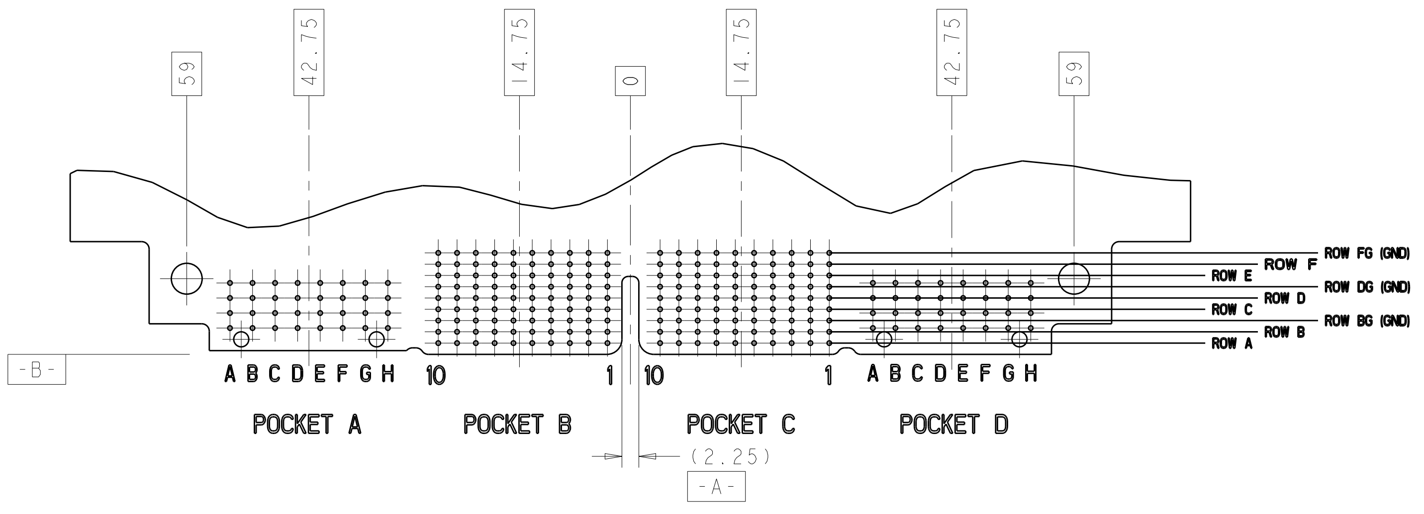
2000795-2 CIRCUIT IDENTIFICATION SCALE 2:1
