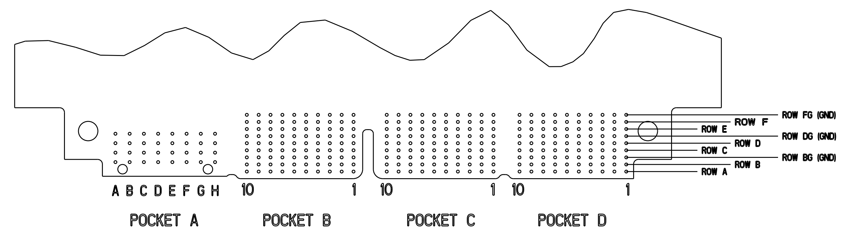
2000795-1 CIRCUIT IDENTIFICATION SCALE 2:1
