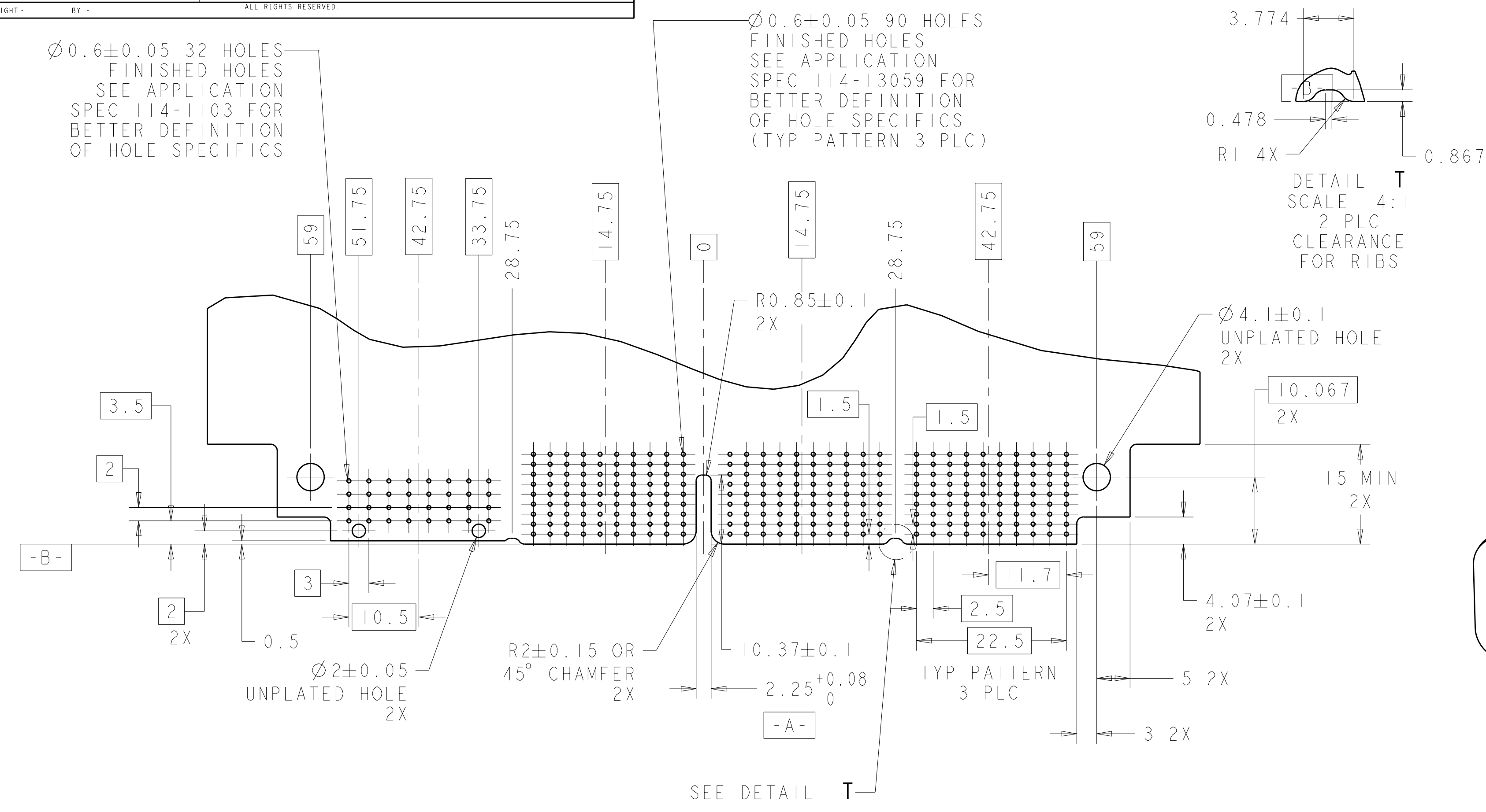
RECOMMENDED PRINTED CIRCUIT BOARD HOLE LAY-OUT AS VIEWED FROM TOP OF PRINTED CIRCUIT BOARD 2000795-1 (3 HMZd AND 1 UPM MODULE)
