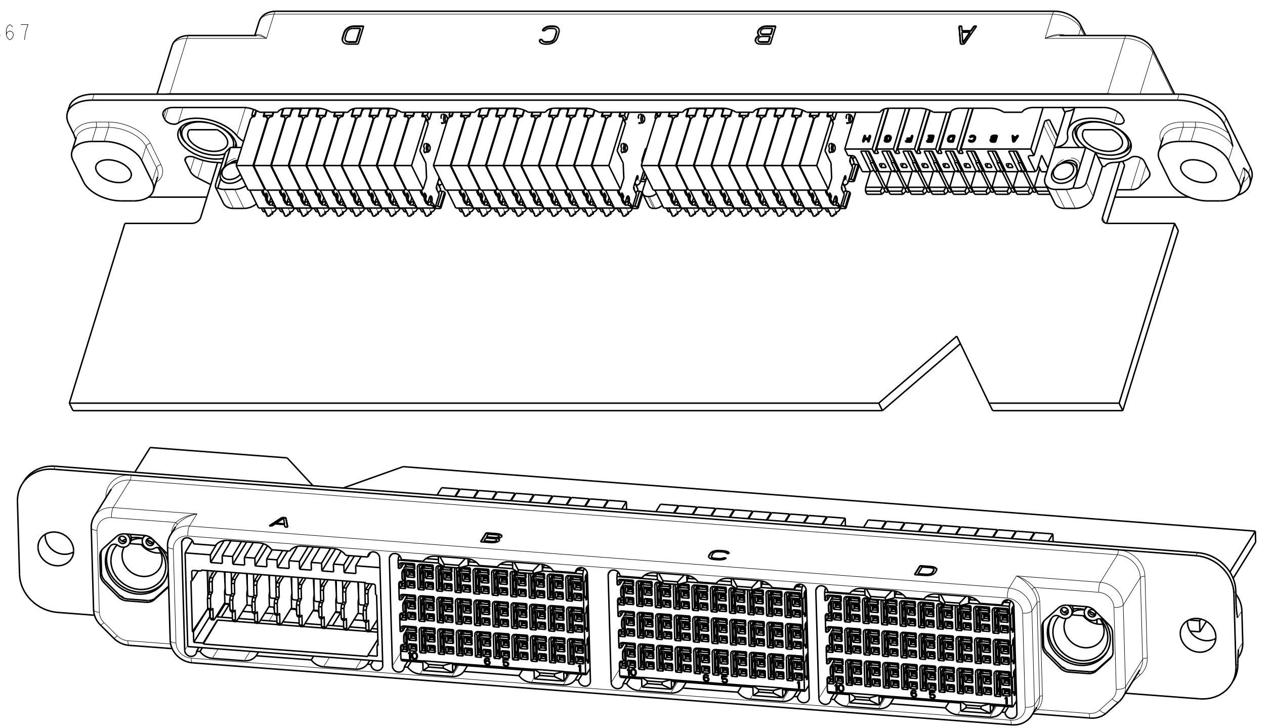
2000975-1 MODULE CONFIGURATION
