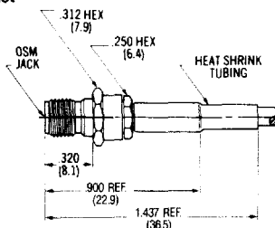
Straight Cable Jack Captured Contact
