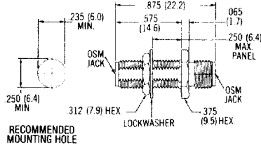
Jack to Jack Adapter Bulkhead Feedthrough
