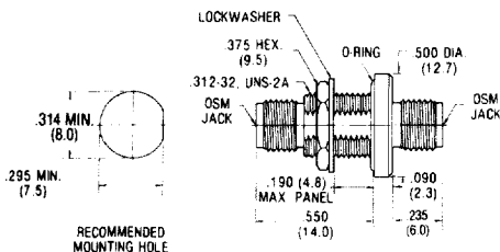
Jack to Jack
