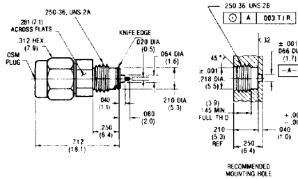
Plug Receptacle
