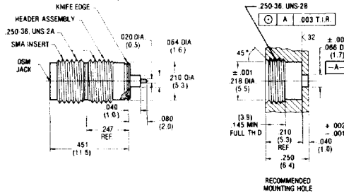
Two-Piece Jack Receptacle
