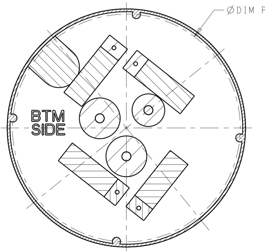
COMPONENT KEEP OUT AREAS 2213871-1, 2213871-2 AND 2213871-3
