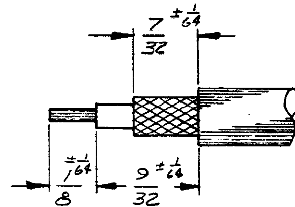
STRIP LENGTH
