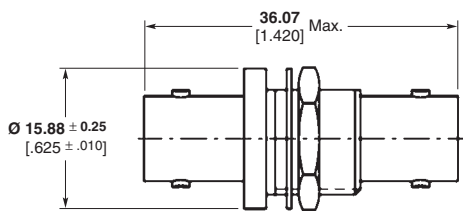
Part No. 1274935-1
