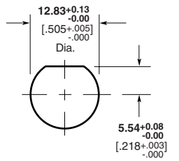
Maximum Panel Thickness 6.35 [0.250] Recommended Panel Cutout
