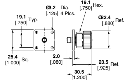
Part No. 1061750-1
