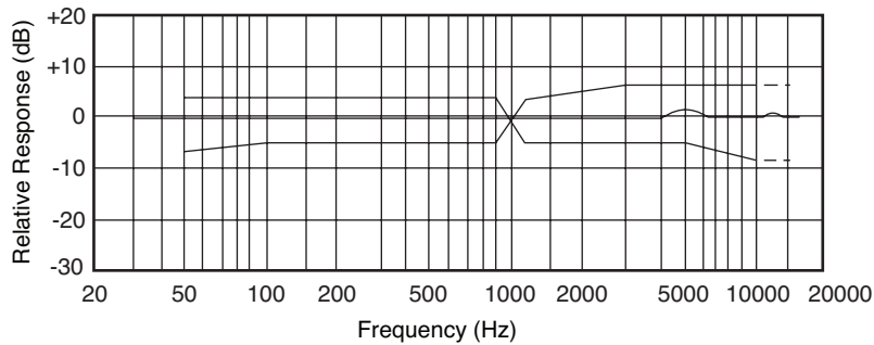
Typical Frequency Response Curve Limit
