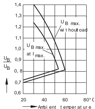
Relay operation voltage vs. ambient temperature
