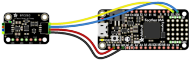
fritzing
