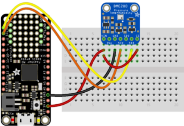
fritzing
