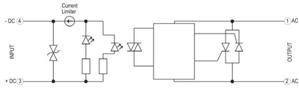
GNA Series DC control / Thyristor 40 A / 50 A / 90 A
