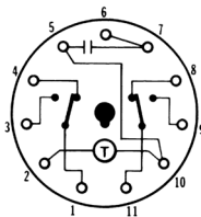
INTERVAL/ON-DELAY
