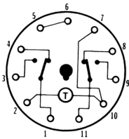
OFF DELAY
