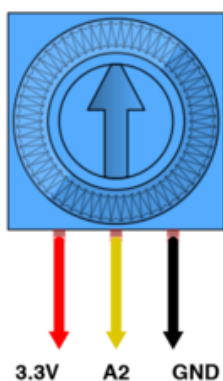
Potentiometer (10K)
