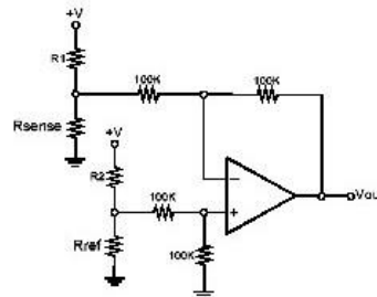
Differential Op-Amp
