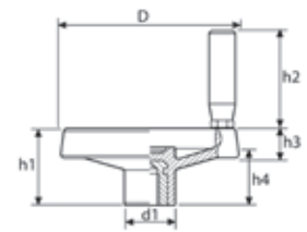
Type 2: With Handle
