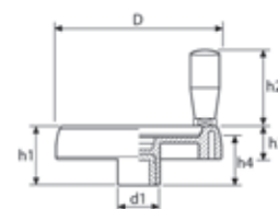
Type 1: With Upright Handle
