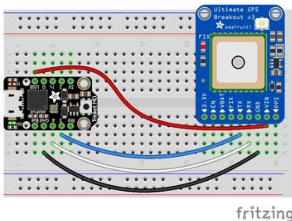
Trinket M0
