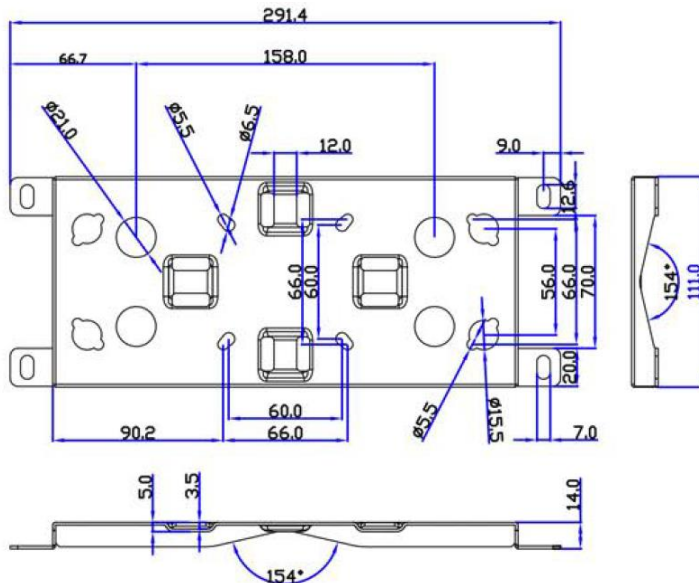
Figure 54: Wall mount dimensions
