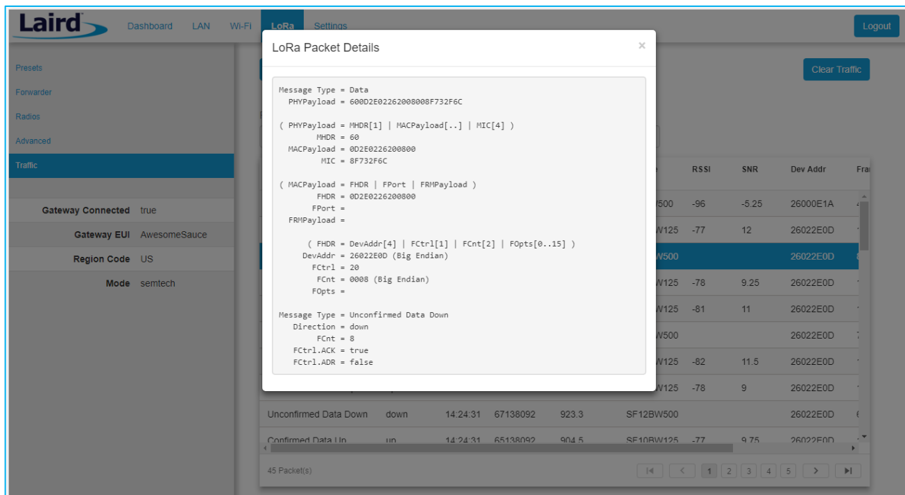
Figure 37: LoRa packet details
