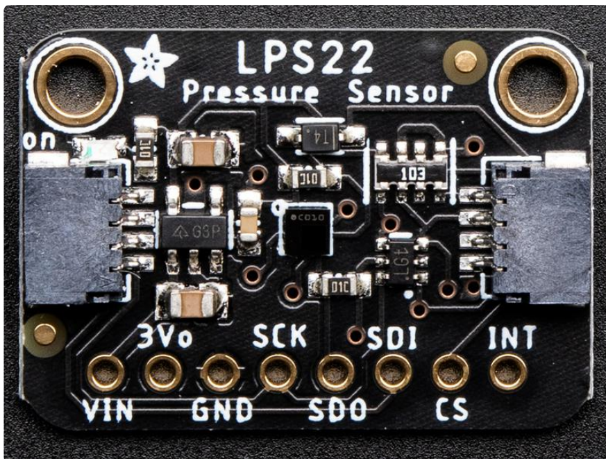
The LPS25 and LPS22 breakouts have identical pinouts; both boards are shown for reference
