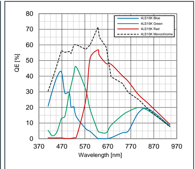
Figure 22: 4LS RGB + Monochrome QE (1)(2)(3)
