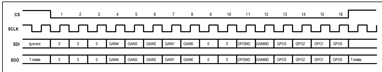
Figure 5. SPI Command Format
