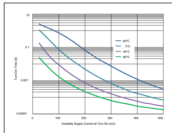
Figure 8. 5173 nominal turn-on time versus available supply current and temperature
