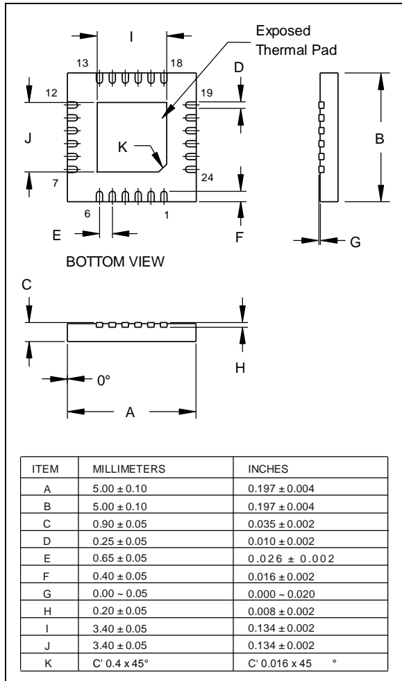
Figure 15. 5 x 5mm QFN-24 Package Dimensions.
