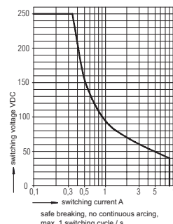
Limit curve for arc-free operation safe breaking, no continuous arcing, max. 1 switching cycle / s
